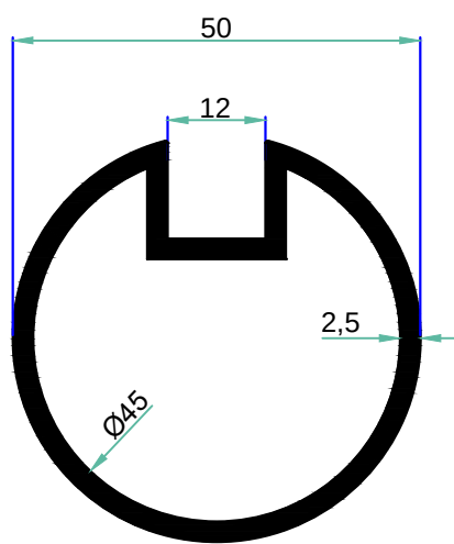
4254 1.163 kg/m
